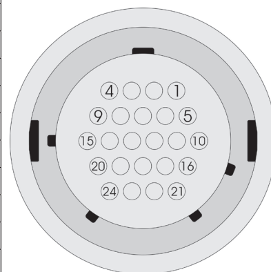
24-way CPC connector - Front view
