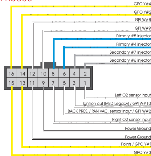
16-way connector rear view
