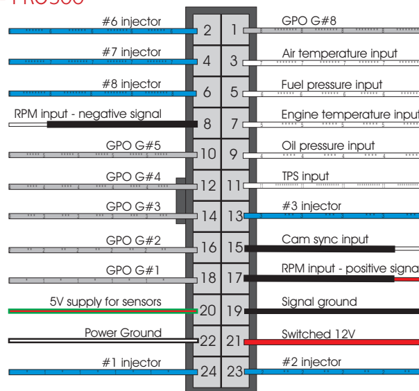
24-way connector rear view
