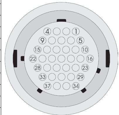
37-way CPC connector - Front view
