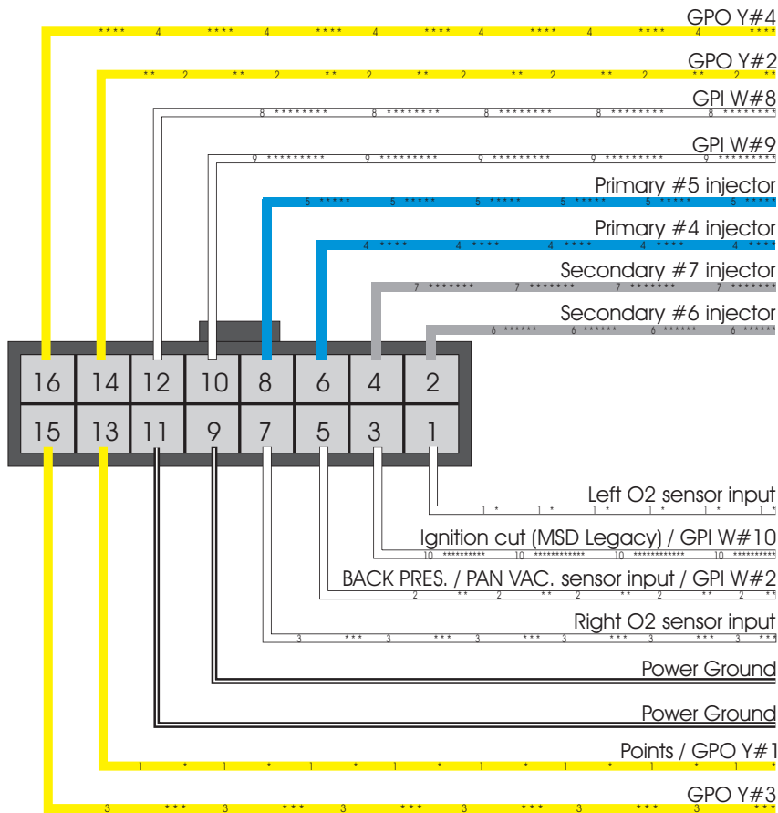
16-way connector rear view
