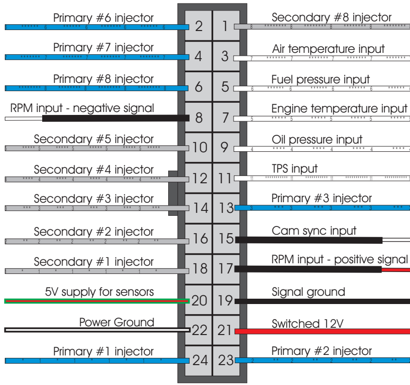
24-way connector rear view
