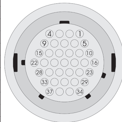
37-way CPC connector - Front view
