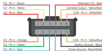
Harness Connector Rear View
